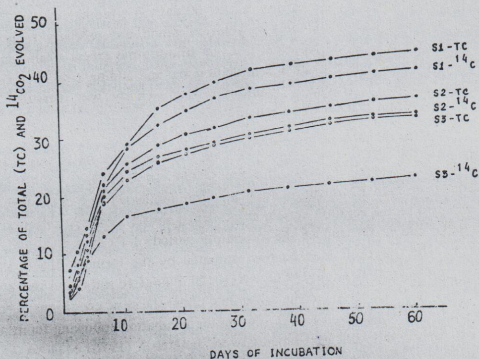
Fig. 1. Decomposition of ^{14}\text{C} labelled Kallar grass during incubation in soil. S1 = Normal soil; S2 = Saline soil; S3 = Saline sodic soil; TC = Total carbon.
