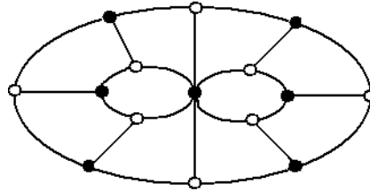
Figure 4: 2-Halin graph
