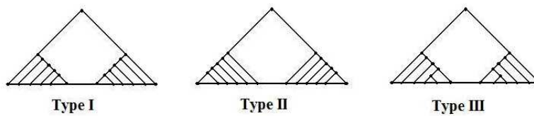
Figure 8: ( m = 12 )
