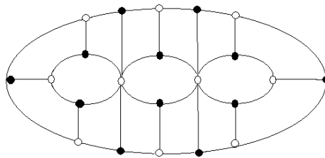
Figure 7: 3-Halin graph
