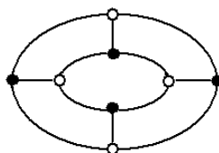
Figure 3: 1-Halin graph
