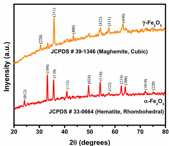
Fig. 2. The comparison of the XRD patterns of \alpha - and \gamma - \text{Fe}_2\text{O}_3 in the range of 2\theta = 20 – 80^\circ .
