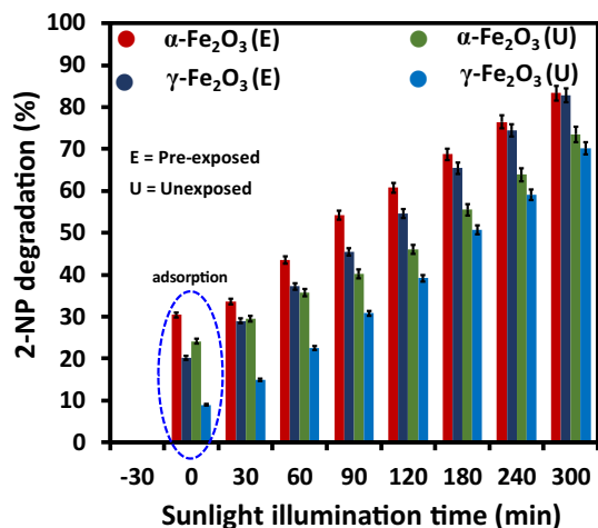
Fig. 12. The comparison of the photocatalytic activity of exposed and unexposed \alpha -Fe 2 O 3 and \gamma -Fe 2 O 3 for the degradation of 2-NP in the exposure of the visible region of sunlight.
