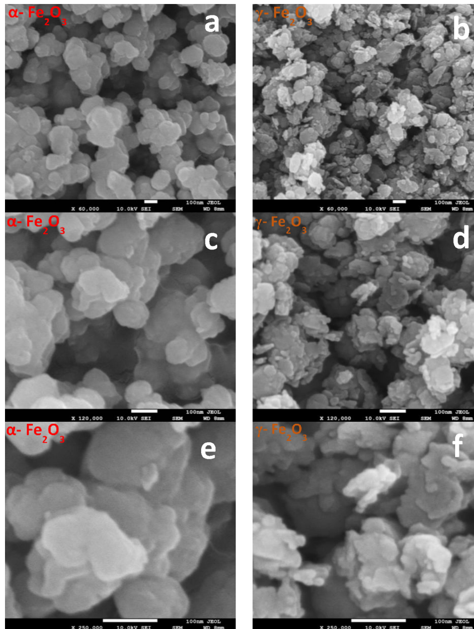
Fig. 3. The comparison of FESEM images of \alpha - \text{Fe}_2\text{O}_3 and \gamma - \text{Fe}_2\text{O}_3 at (a, b) 60kx, (c, d) 120kx and (e, f) 250kx, respectively.
