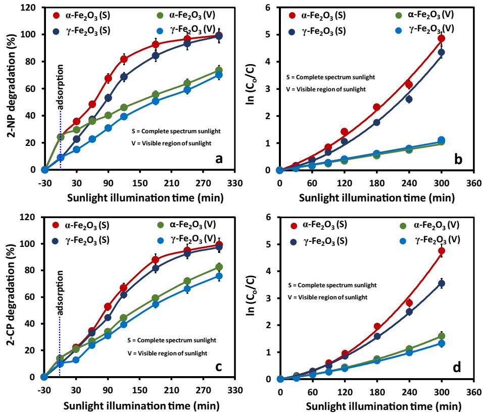
Fig. 7. The comparison of the percentage degradation (a, c) and plots of \ln(C_0/C) versus sunlight exposure time (b, d) of 2-NP and 2-CP respectively, over \alpha - and \gamma -Fe 2 O 3 .
