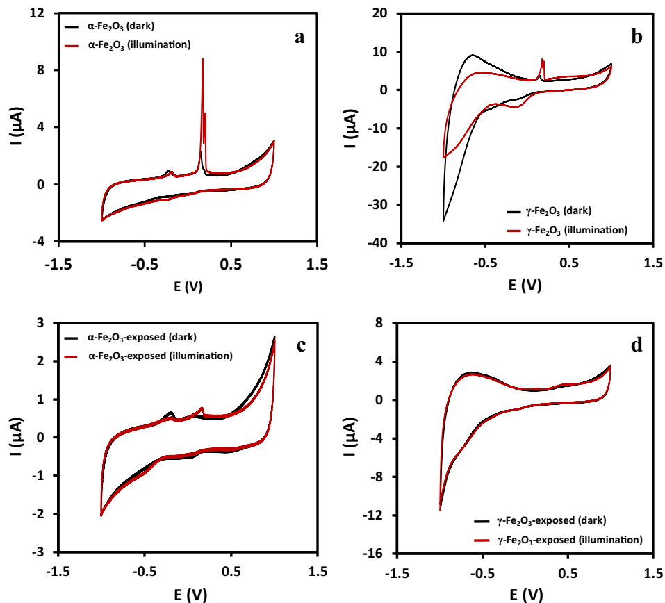
Fig. 10. The comparison of the CV profiles (a) unexposed \alpha -Fe 2 O 3 , (b) unexposed \gamma -Fe 2 O 3 , (c) exposed \alpha -Fe 2 O 3 and (d) exposed \gamma -Fe 2 O 3 in the dark and under illumination.
