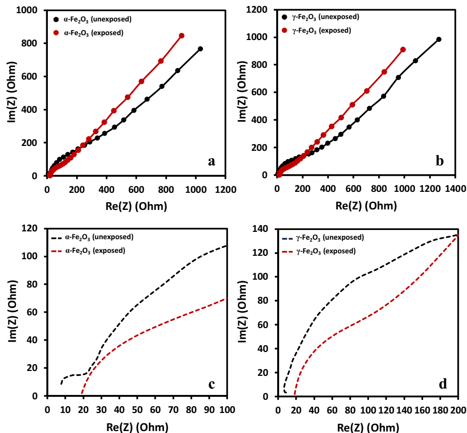
Fig. 11. The comparison of the EIS Nyquist plots of exposed and unexposed (a, c) \alpha -Fe 2 O 3 (b, d) \gamma -Fe 2 O 3 in the high and low-frequency linear region under illumination.
