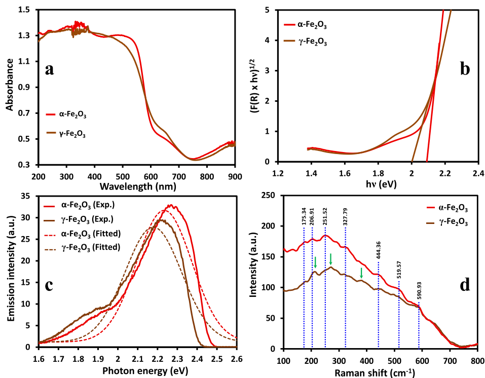
Fig. 1. The comparison of the (a) solid-state absorption spectra in 200–900 nm range, (b) graphical evaluation of bandgap, (c) PL spectra and (d) Raman spectra of \alpha - and \gamma -Fe 2 O 3 .
