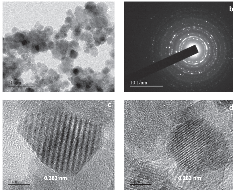
Fig. 5. (a) The HRTEM image, (b) the SAED patterns corresponding to the identified discrete spacing and (c, d) the identified discrete spacing of 0.283 nm in two different crystals of \gamma -Fe 2 O 3 .
