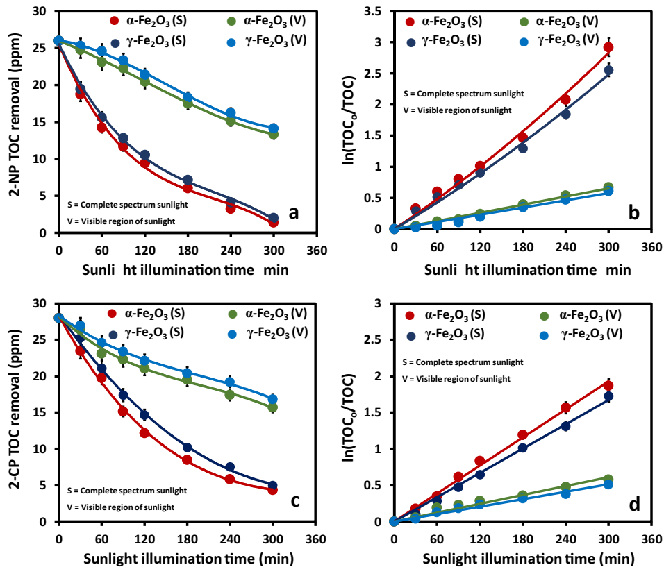
Fig. 8. The comparison of decrease in TOC removal (a, c) and plots of \ln(TOC_0/TOC) versus the sunlight exposure time (b, d) 2-NP and 2-CP over \alpha - and \gamma -Fe 2 O 3 in sunlight exposure.
