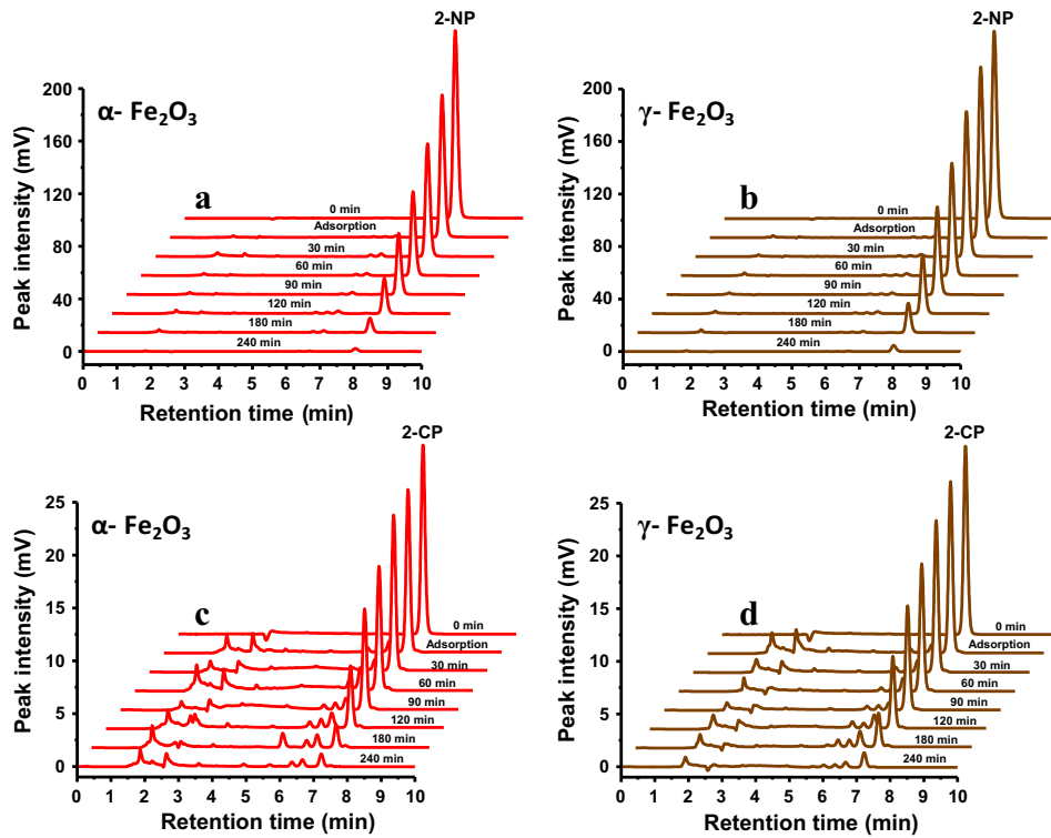
Fig. 9. The comparison of HPLC degradation profiles (a) 2-NP, \alpha -Fe 2 O 3 , (b) 2-NP, \gamma -Fe 2 O 3 , (c) 2-CP, \alpha -Fe 2 O 3 and (d) 2-CP, \gamma -Fe 2 O 3 in complete spectrum sunlight exposure.
